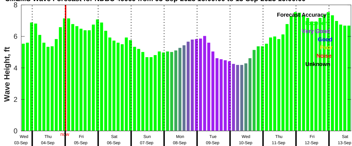
CMEMS Wave Forecast for NDBC 46069 from 03-Sep-2025 16:00:00 to 13-Sep-2025 16:00:00
