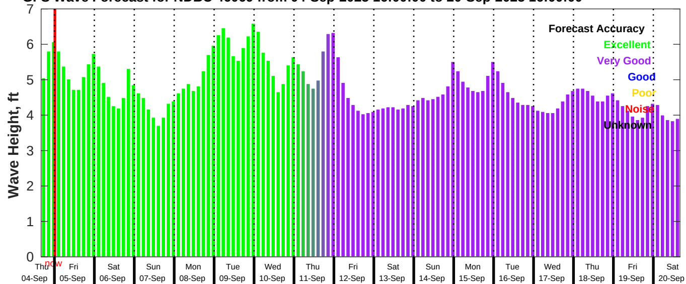
GFS Wave Forecast for NDBC 46069 from 04-Sep-2025 16:00:00 to 20-Sep-2025 16:00:00
