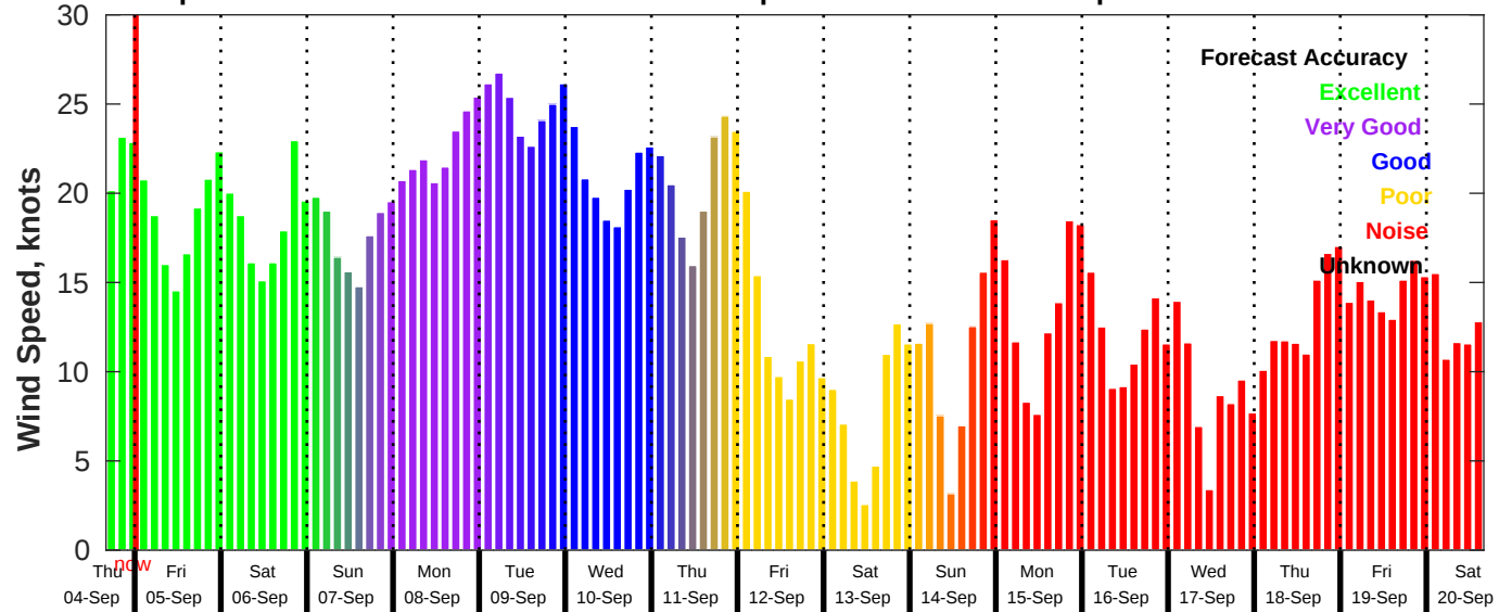
GFS Wind Speed Forecast for NDBC 46069 from 04-Sep-2025 16:00:00 to 20-Sep-2025 16:00:00
