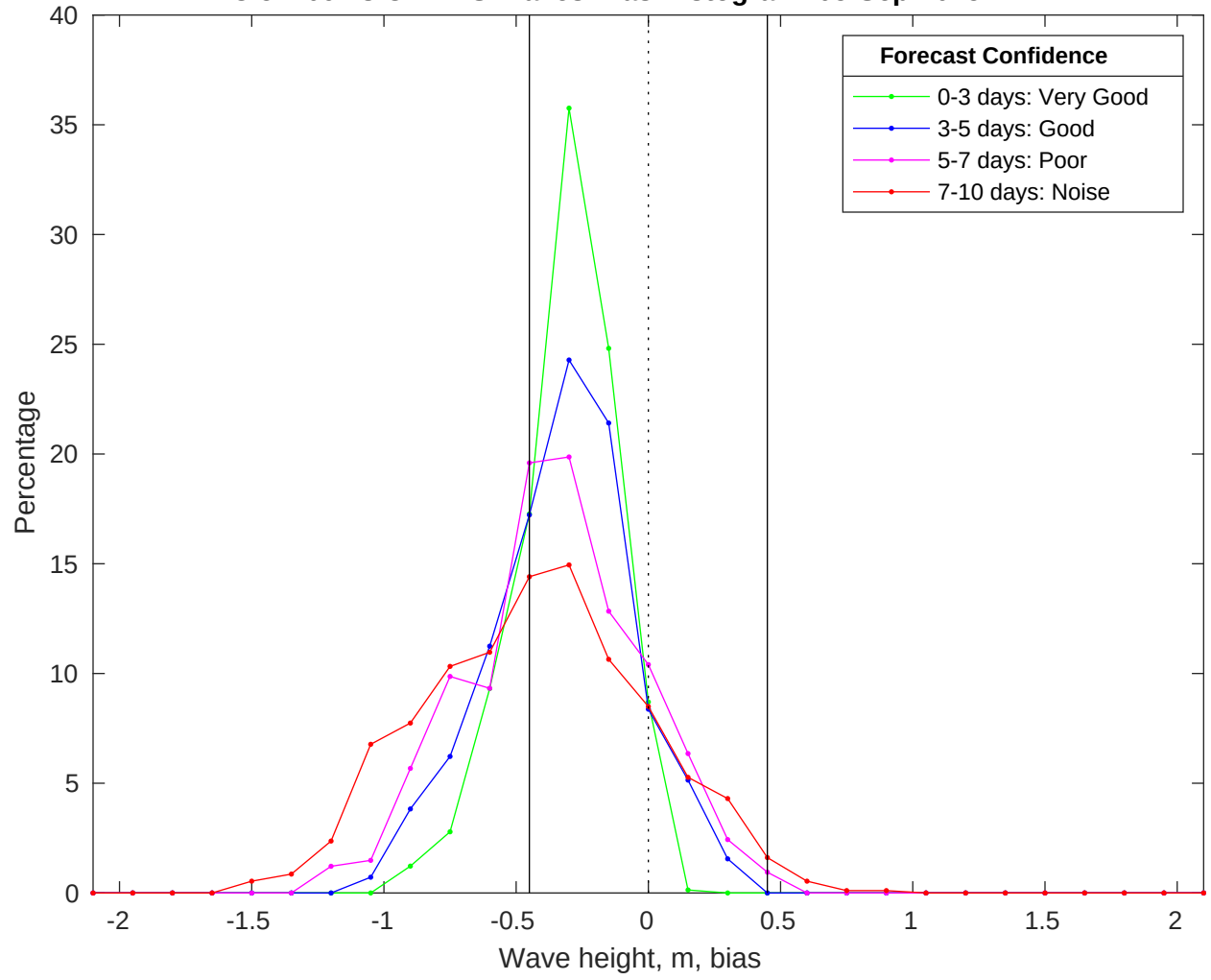
NDBC 51209 vs CMEMS Waves Bias Histogram: 05-Sep-2025
