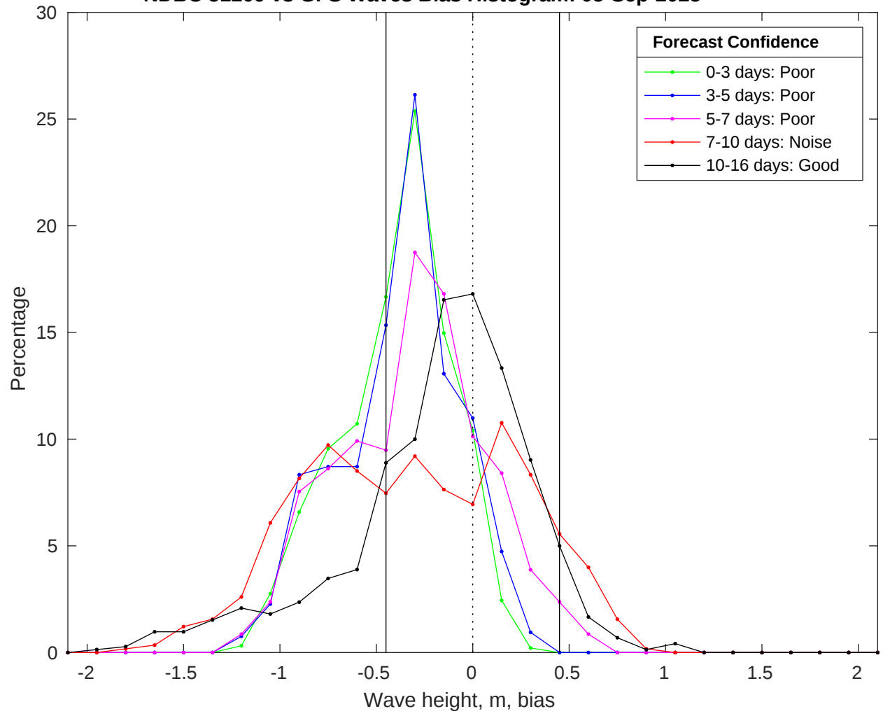
NDBC 51209 vs GFS Waves Bias Histogram: 05-Sep-2025
