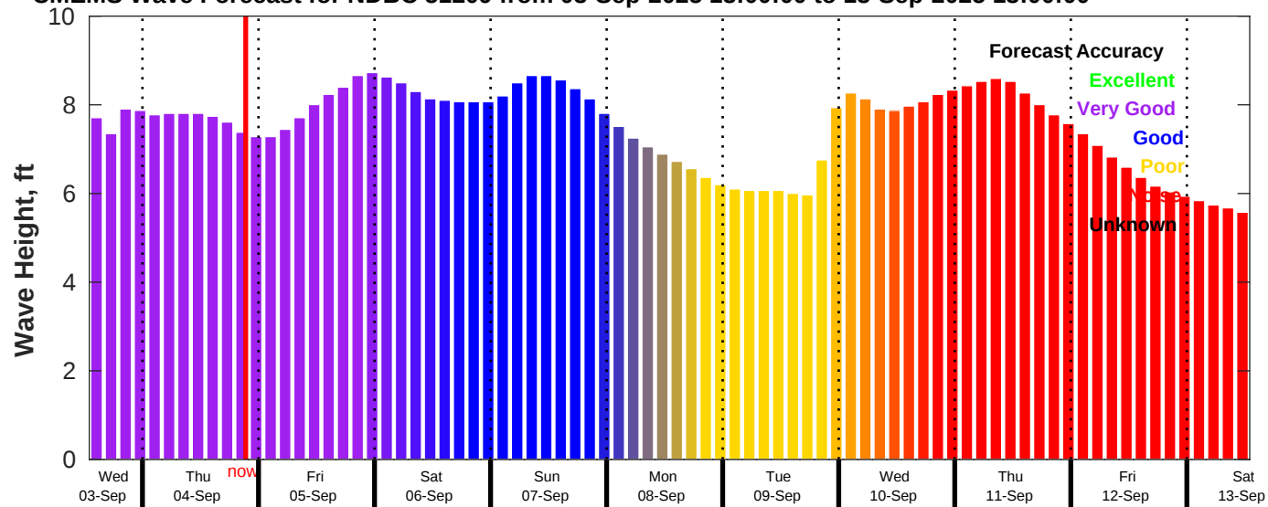
CMEMS Wave Forecast for NDBC 51209 from 03-Sep-2025 13:00:00 to 13-Sep-2025 13:00:00
