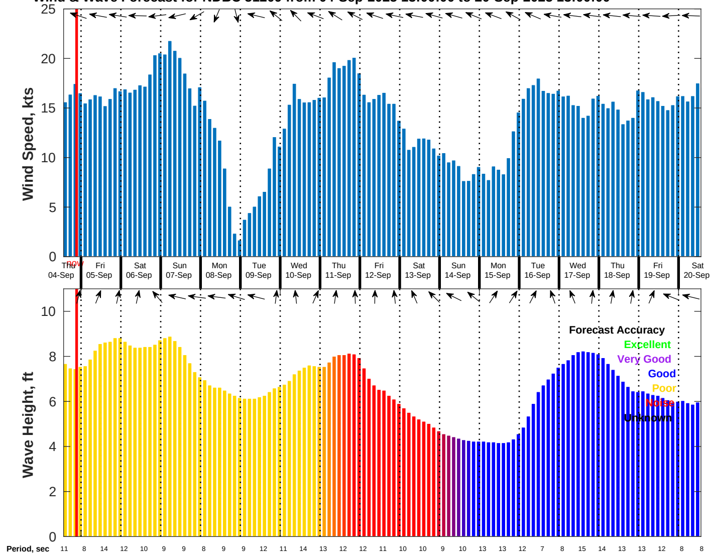
Wind & Wave Forecast for NDBC 51209 from 04-Sep-2025 13:00:00 to 20-Sep-2025 13:00:00
