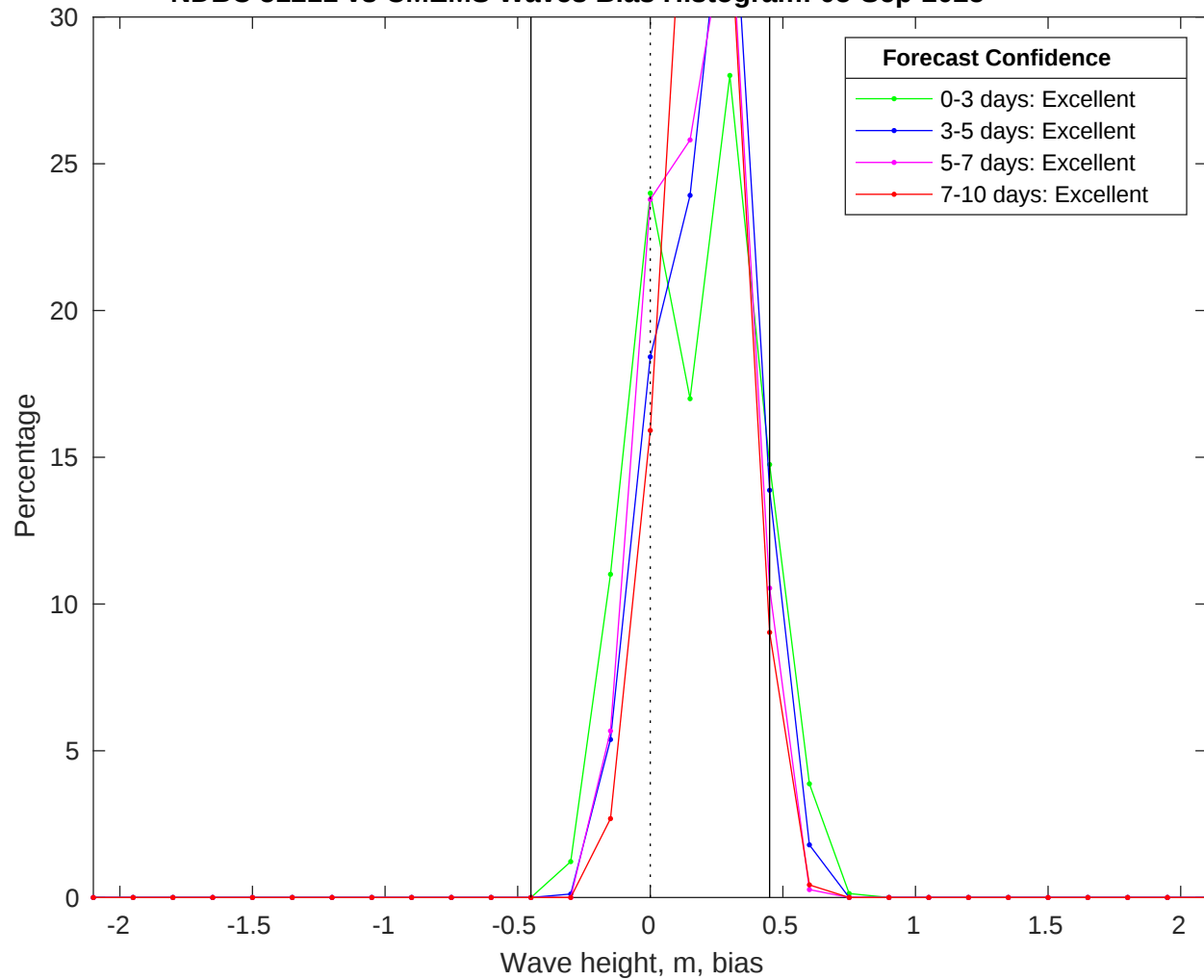
NDBC 51211 vs CMEMS Waves Bias Histogram: 05-Sep-2025
