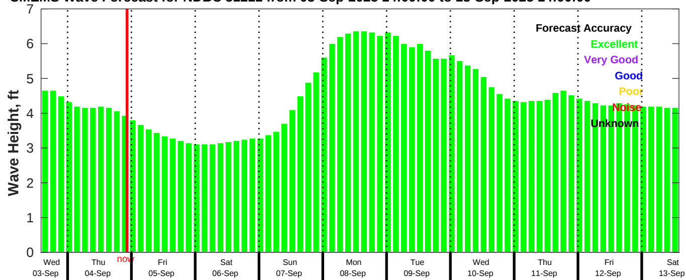
CMEMS Wave Forecast for NDBC 51211 from 03-Sep-2025 14:00:00 to 13-Sep-2025 14:00:00
