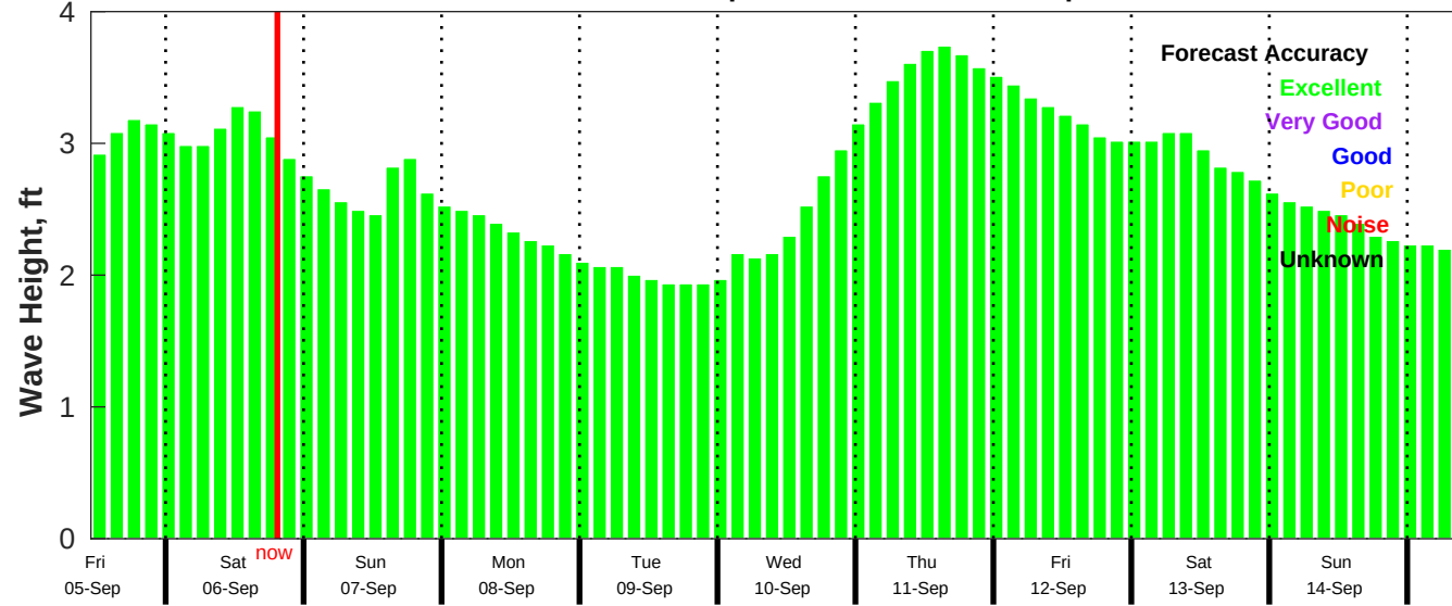
CMEMS Wave Forecast for NDBC 52211 from 04-Sep-2025 11:00:00 to 14-Sep-2025 11:00:00
