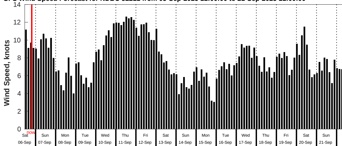
GFS Wind Speed Forecast for NDBC 52211 from 05-Sep-2025 11:00:00 to 21-Sep-2025 11:00:00
