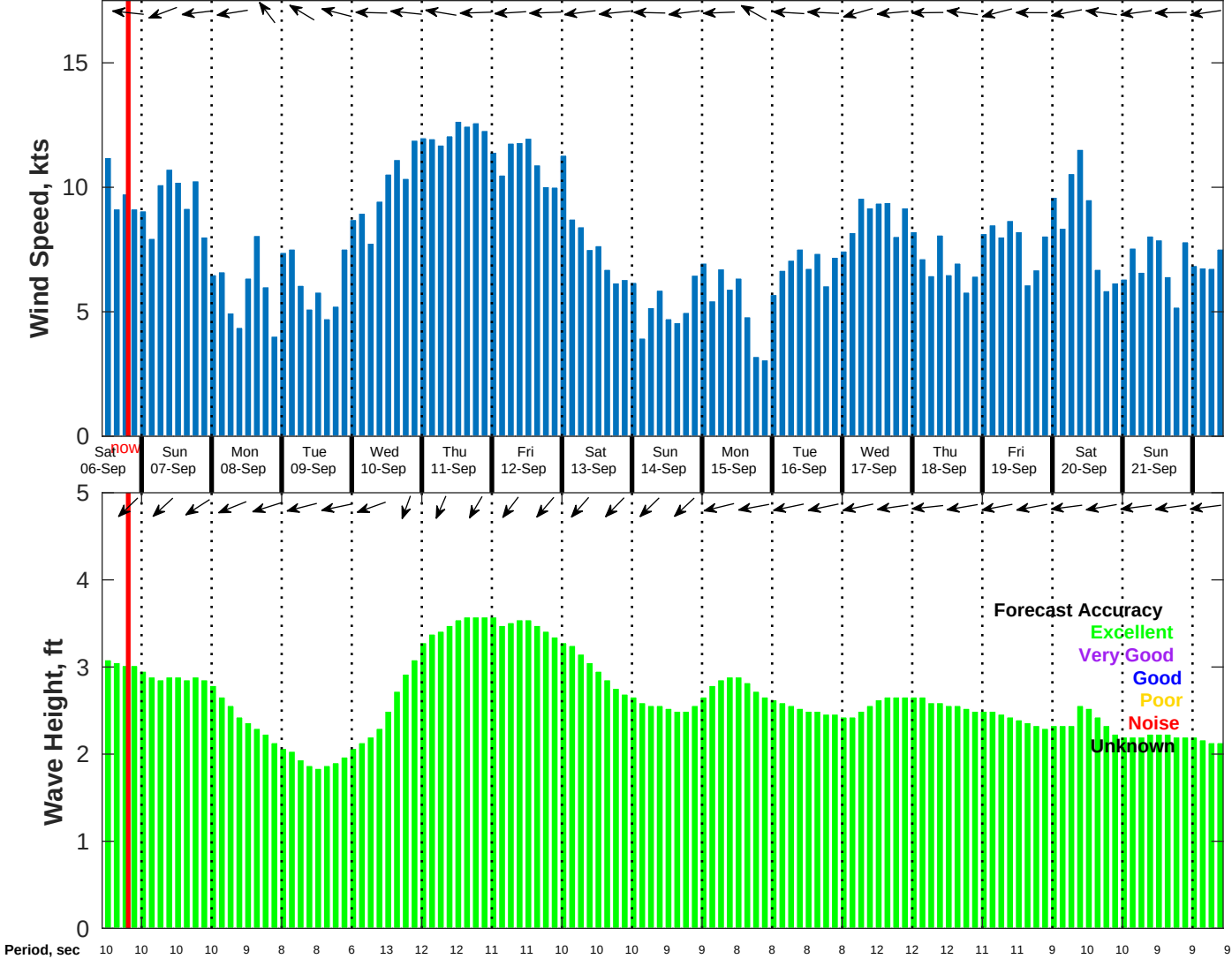
Wind & Wave Forecast for NDBC 52211 from 05-Sep-2025 11:00:00 to 21-Sep-2025 11:00:00
