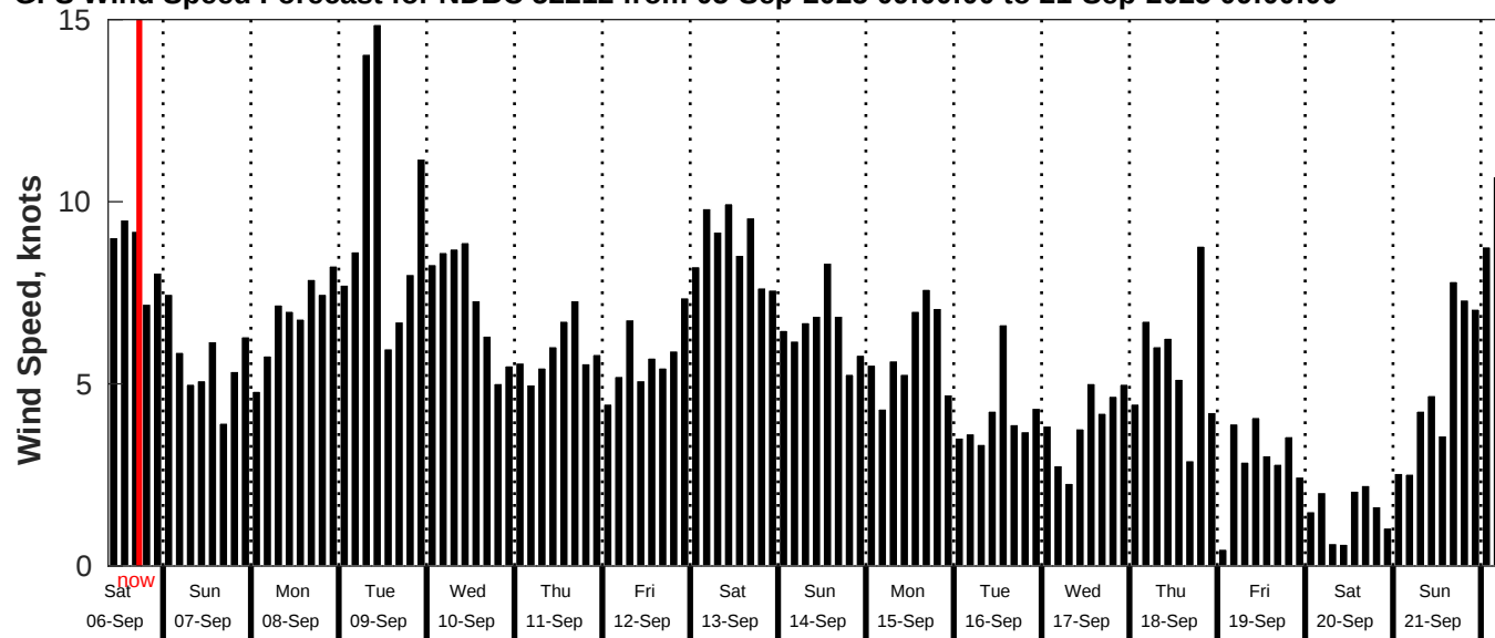
GFS Wind Speed Forecast for NDBC 52212 from 05-Sep-2025 09:00:00 to 21-Sep-2025 09:00:00
