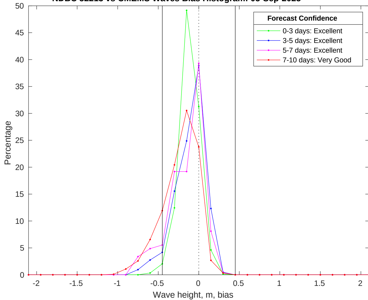
NDBC 52213 vs CMEMS Waves Bias Histogram: 05-Sep-2025
