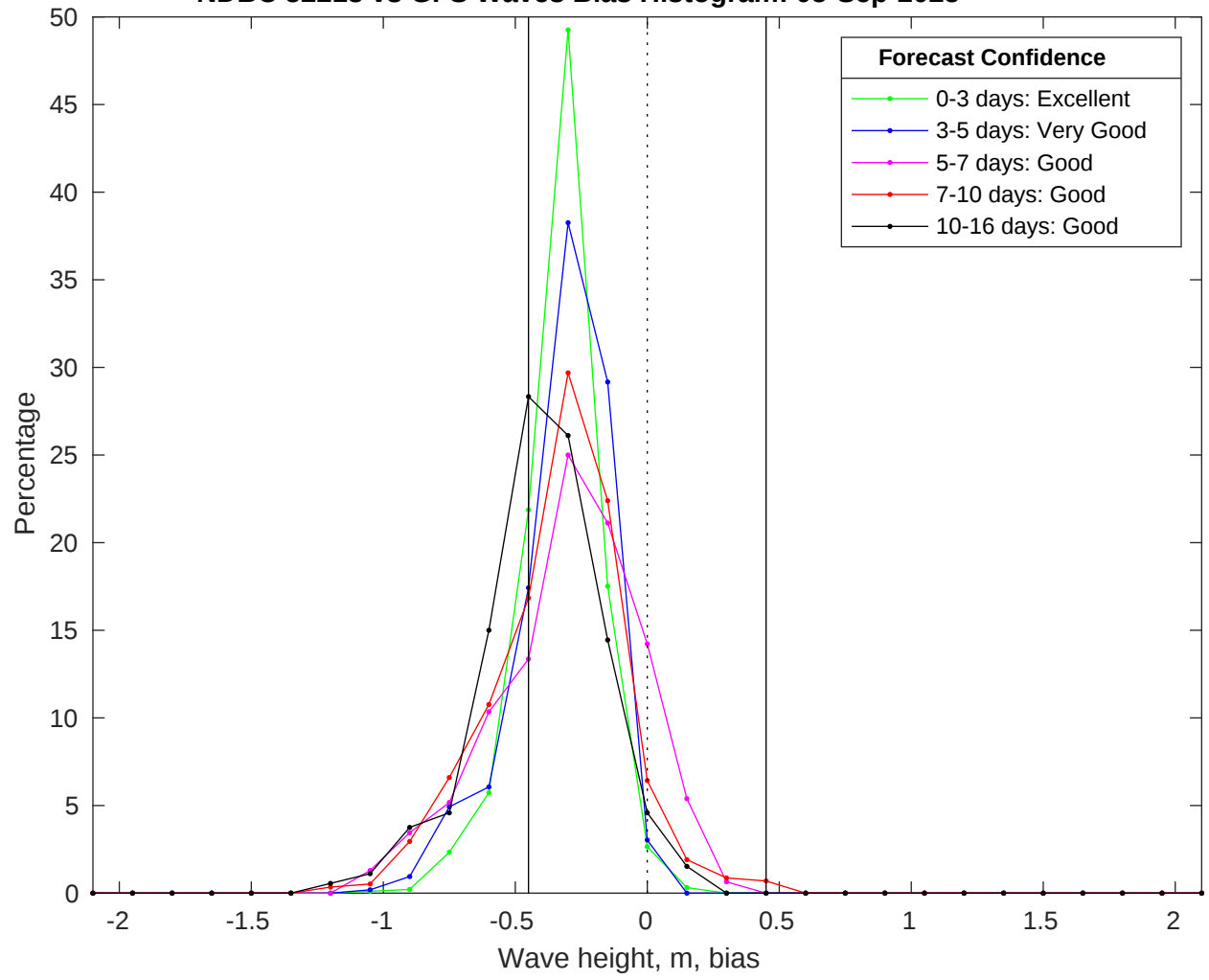
NDBC 52213 vs GFS Waves Bias Histogram: 05-Sep-2025
