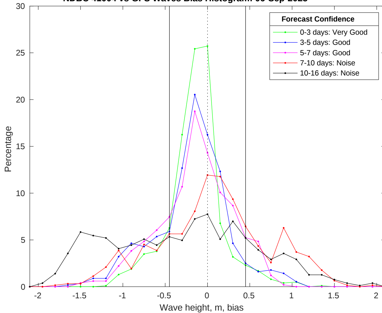
NDBC 41004 vs GFS Waves Bias Histogram: 06-Sep-2025
