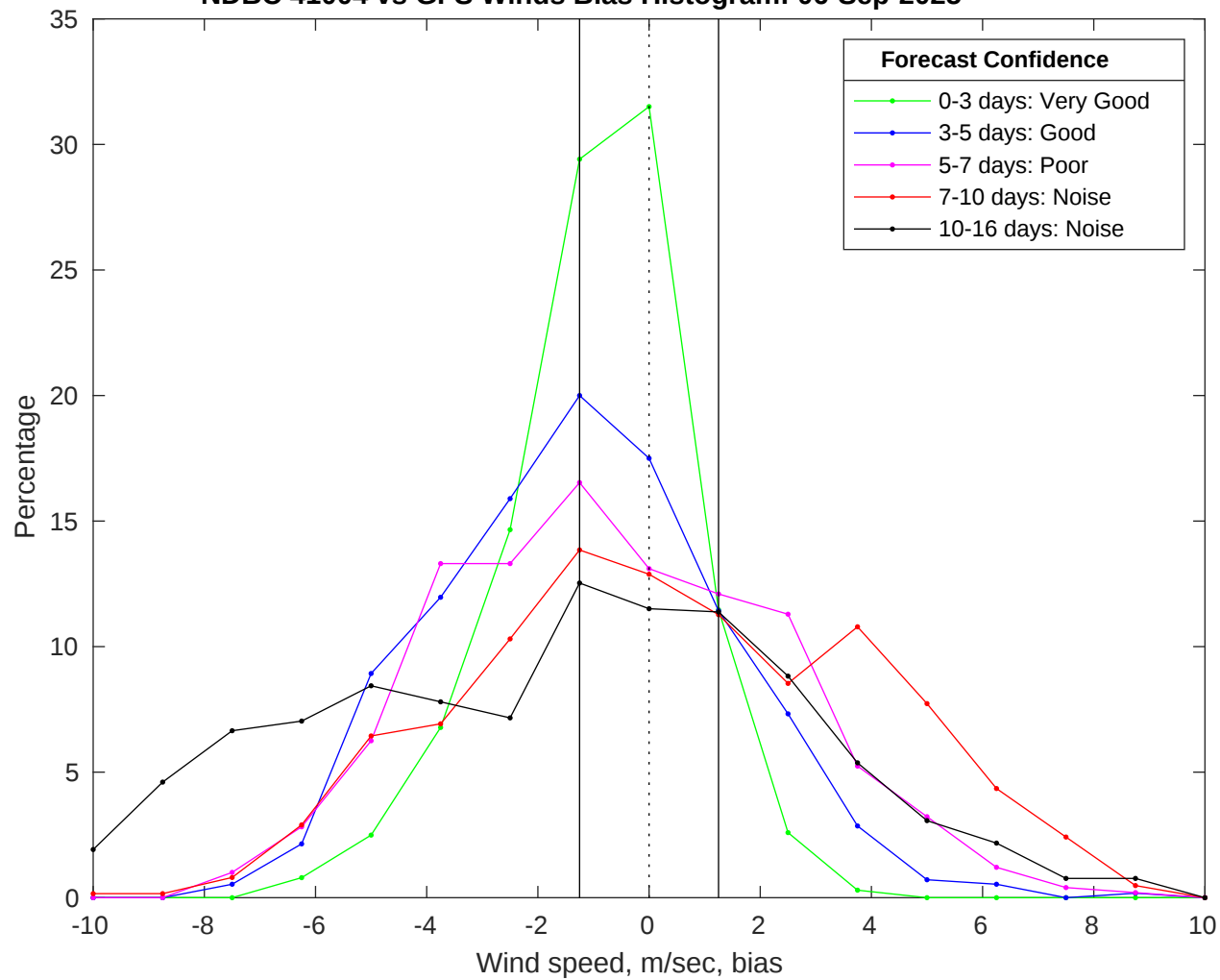
NDBC 41004 vs GFS Winds Bias Histogram: 06-Sep-2025
