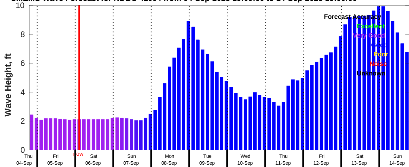
CMEMS Wave Forecast for NDBC 41004 from 04-Sep-2025 19:00:00 to 14-Sep-2025 19:00:00
