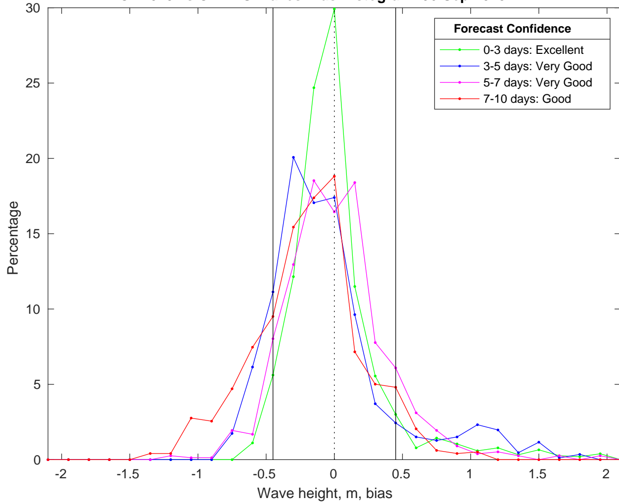
NDBC 41013 vs CMEMS Waves Bias Histogram: 06-Sep-2025
