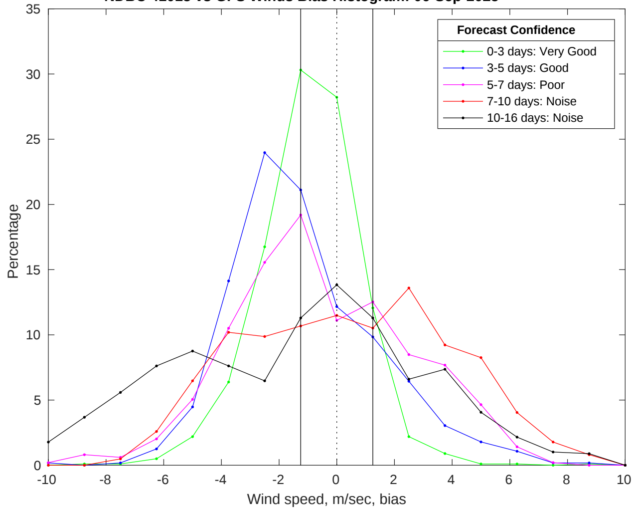
NDBC 41013 vs GFS Winds Bias Histogram: 06-Sep-2025
