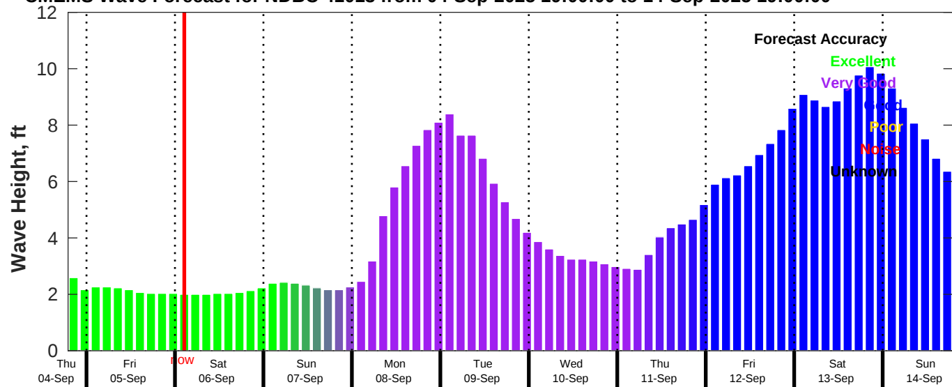
CMEMS Wave Forecast for NDBC 41013 from 04-Sep-2025 19:00:00 to 14-Sep-2025 19:00:00
