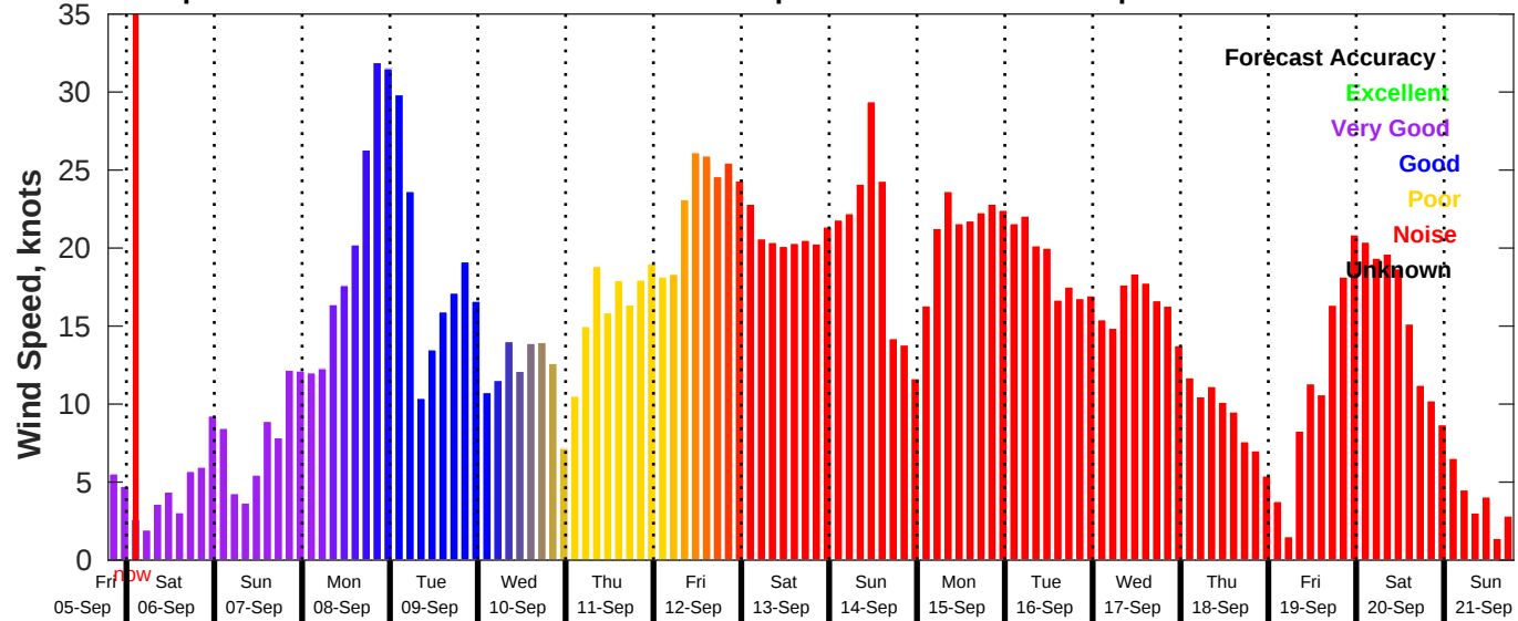
GFS Wind Speed Forecast for NDBC 41013 from 05-Sep-2025 19:00:00 to 21-Sep-2025 19:00:00
