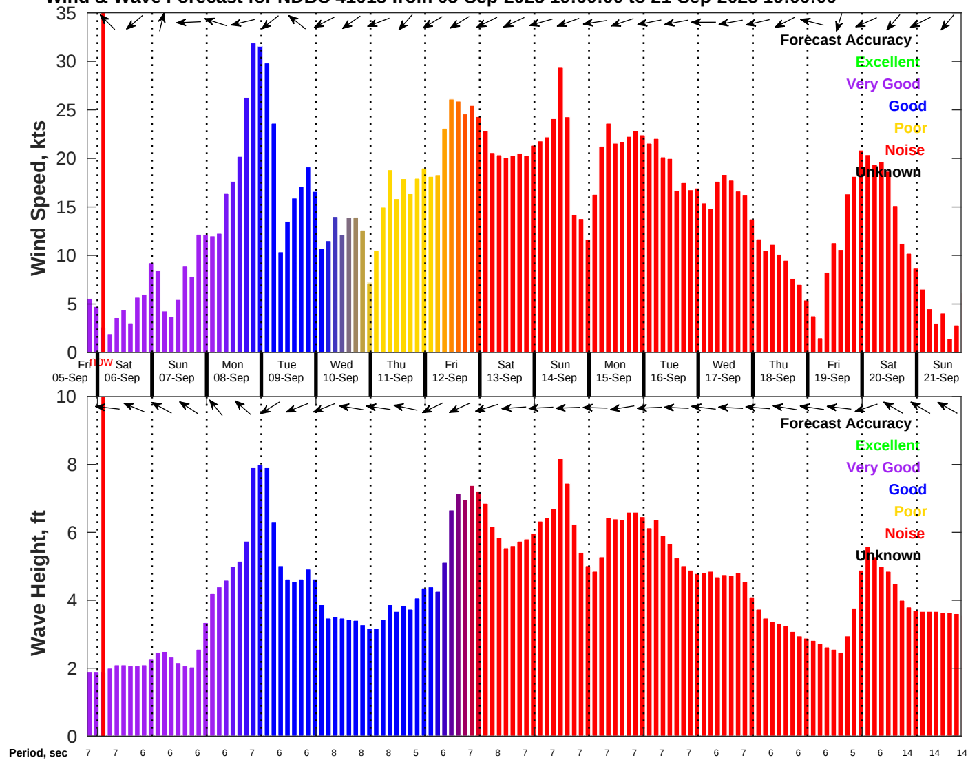
Wind & Wave Forecast for NDBC 41013 from 05-Sep-2025 19:00:00 to 21-Sep-2025 19:00:00
