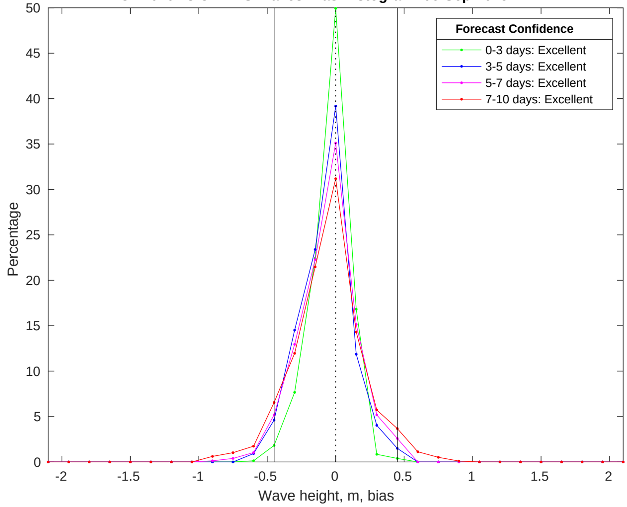
NDBC 41040 vs CMEMS Waves Bias Histogram: 06-Sep-2025
