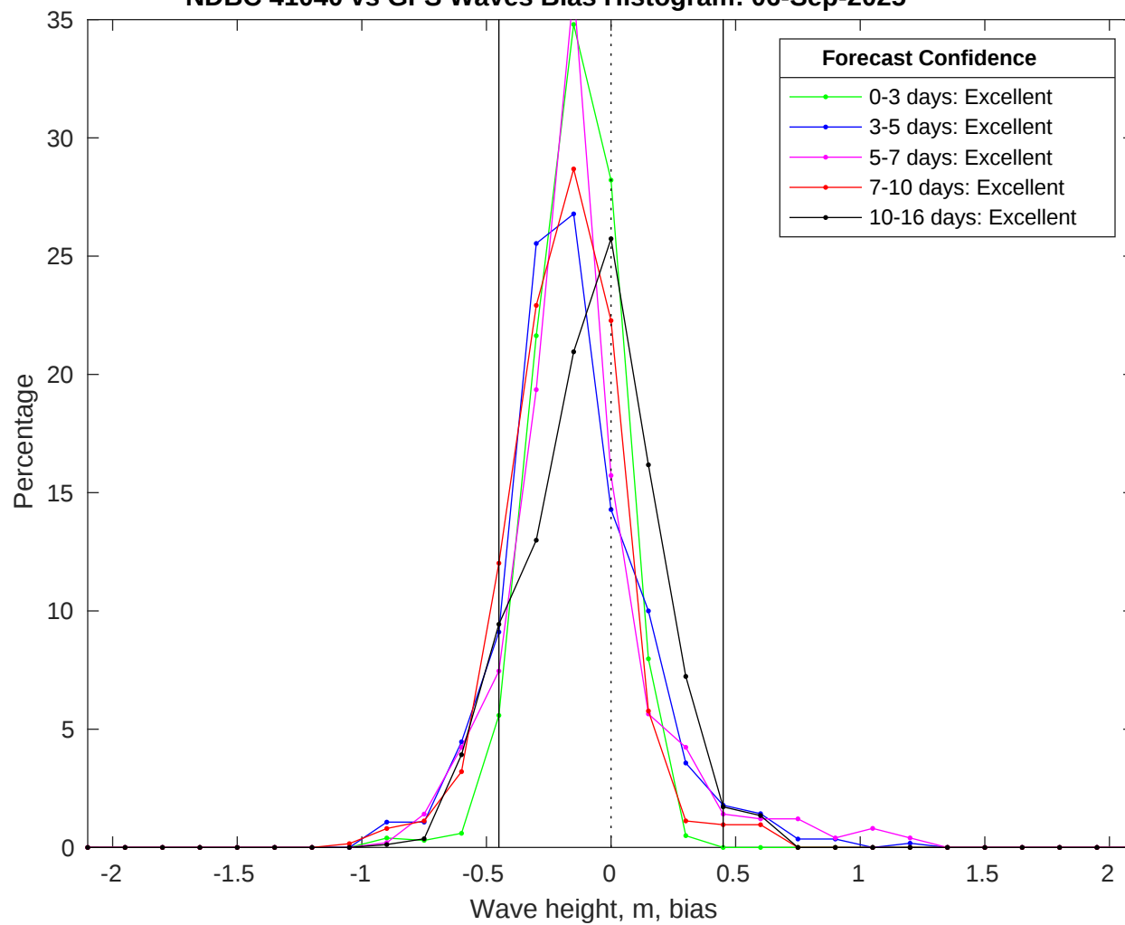
NDBC 41040 vs GFS Waves Bias Histogram: 06-Sep-2025
