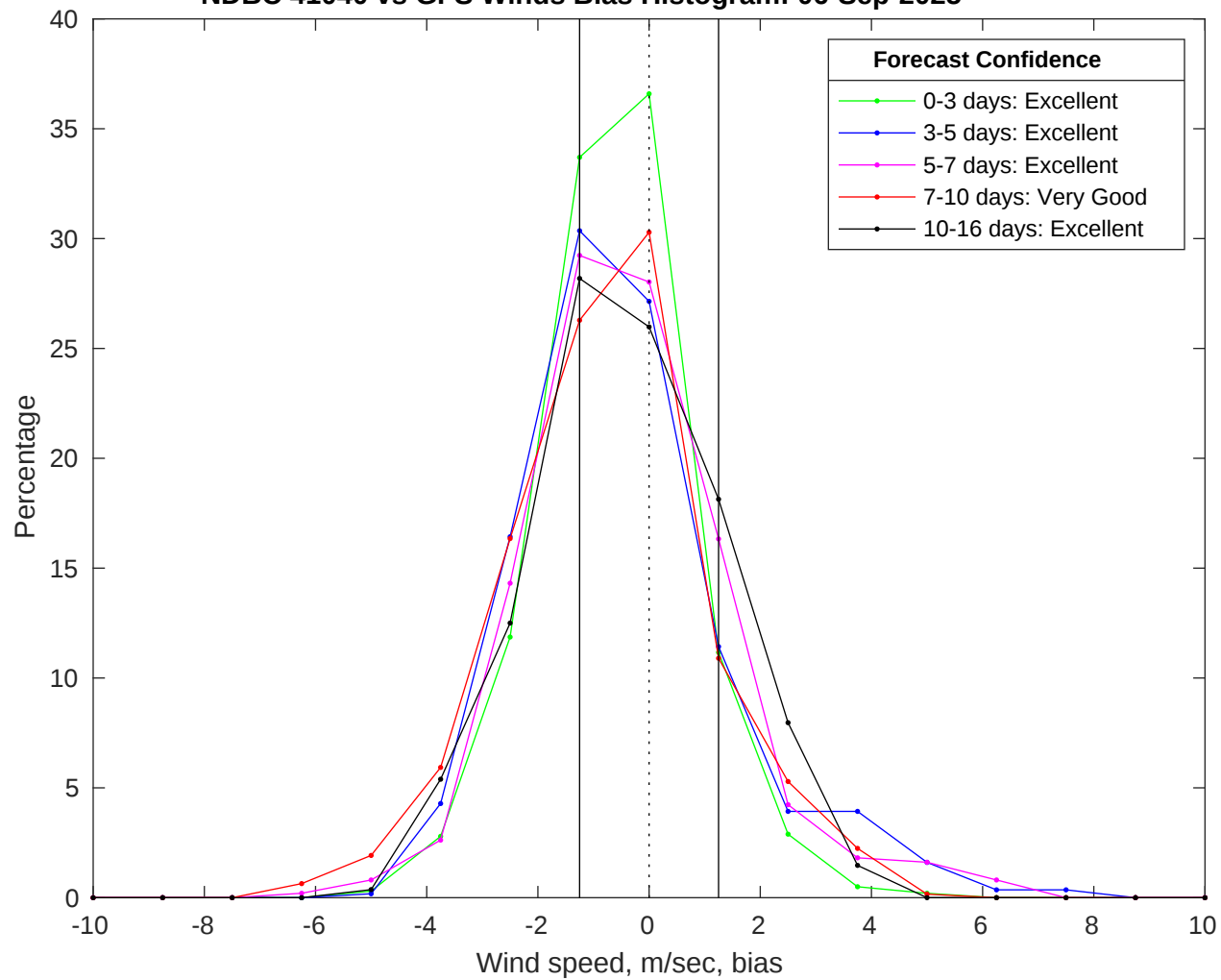
NDBC 41040 vs GFS Winds Bias Histogram: 06-Sep-2025
