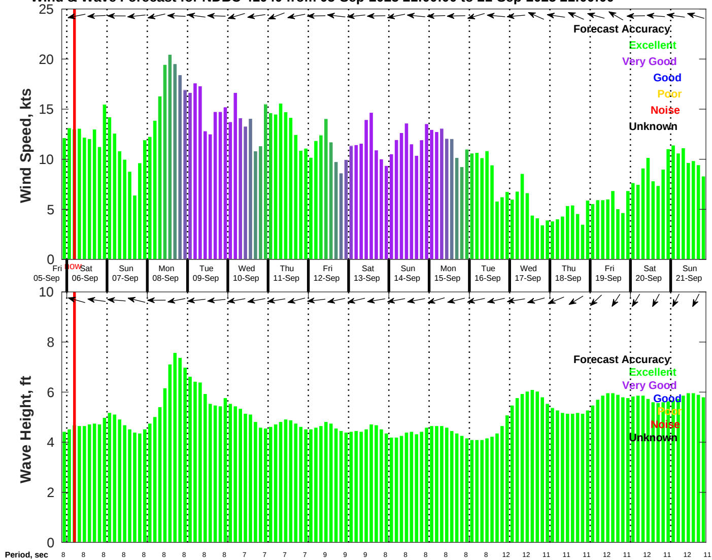
Wind & Wave Forecast for NDBC 41040 from 05-Sep-2025 21:00:00 to 21-Sep-2025 21:00:00
