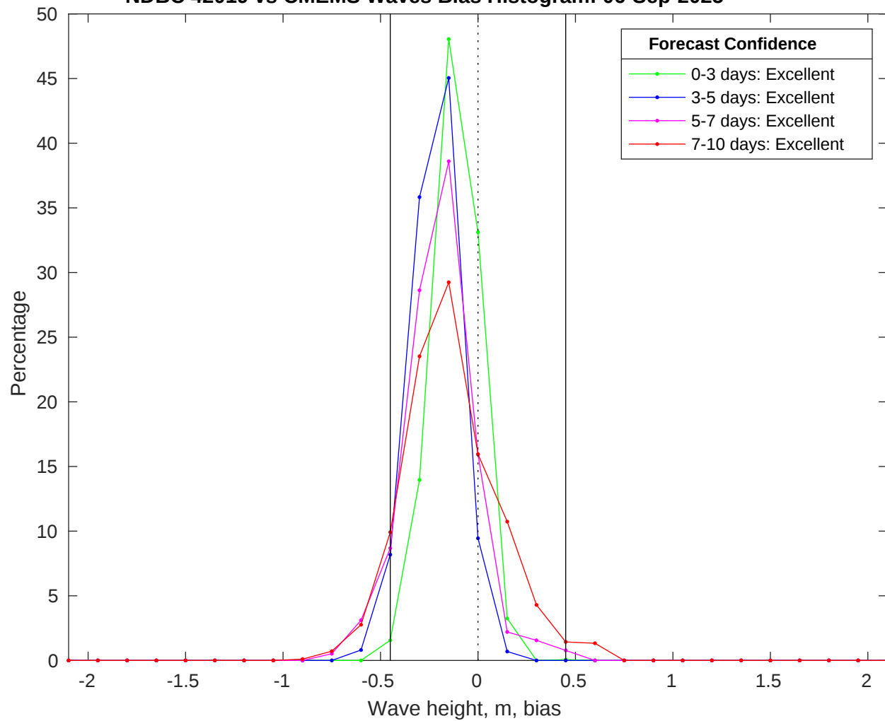
NDBC 42019 vs CMEMS Waves Bias Histogram: 06-Sep-2025
