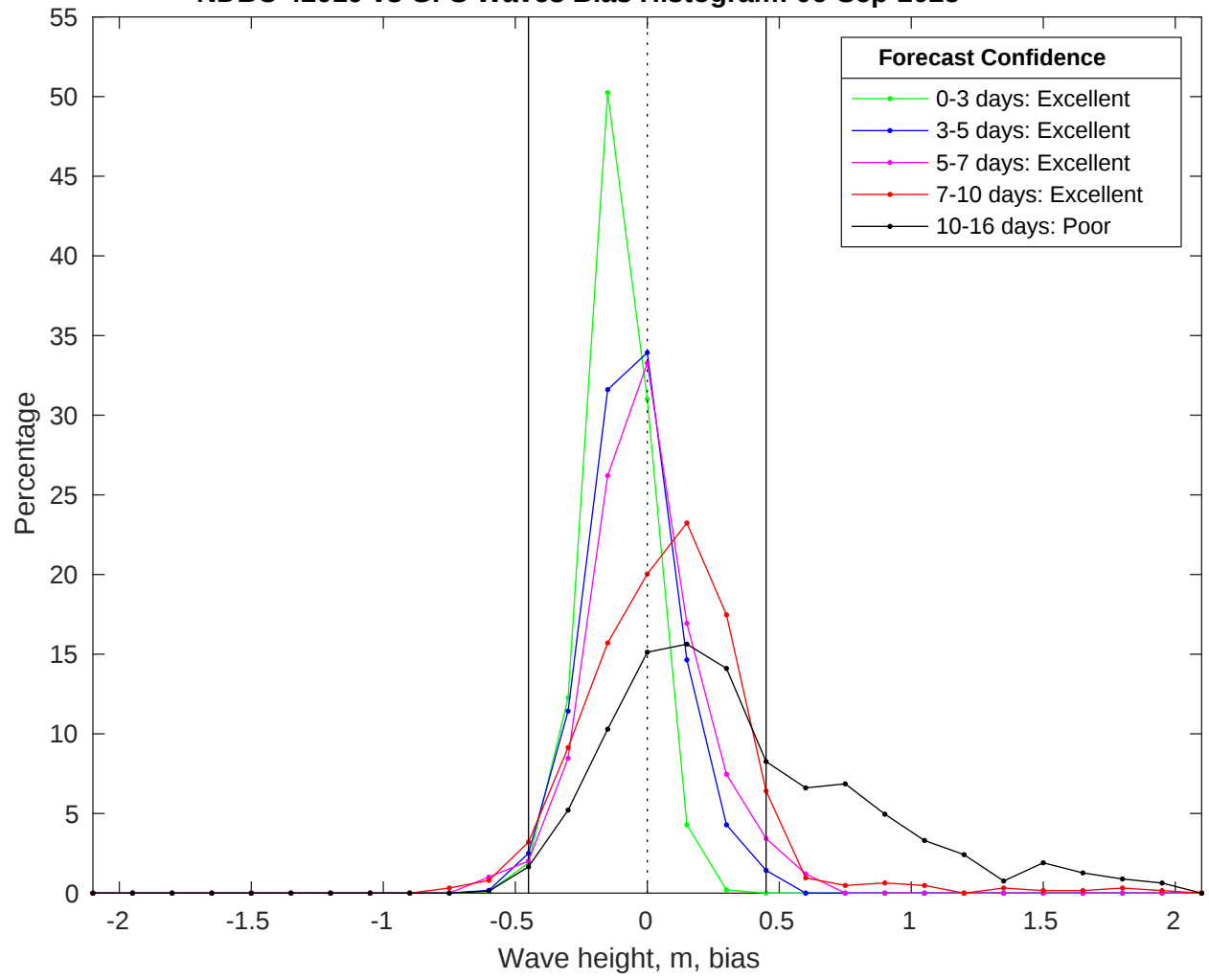
NDBC 42019 vs GFS Waves Bias Histogram: 06-Sep-2025
