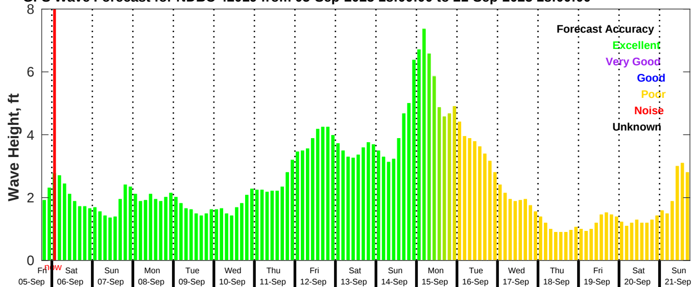
GFS Wave Forecast for NDBC 42019 from 05-Sep-2025 18:00:00 to 21-Sep-2025 18:00:00
