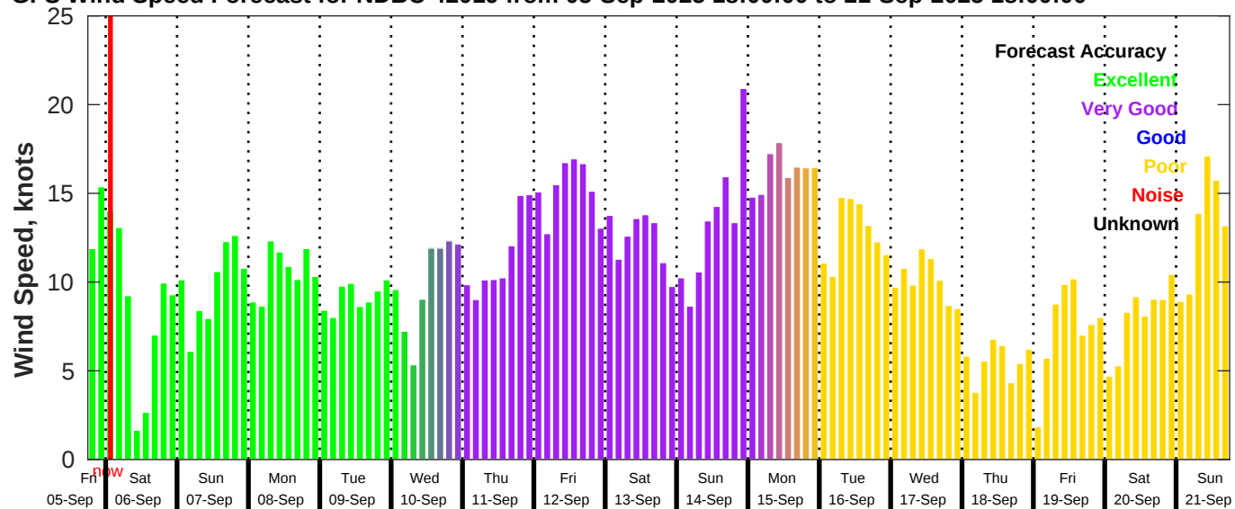
GFS Wind Speed Forecast for NDBC 42019 from 05-Sep-2025 18:00:00 to 21-Sep-2025 18:00:00
