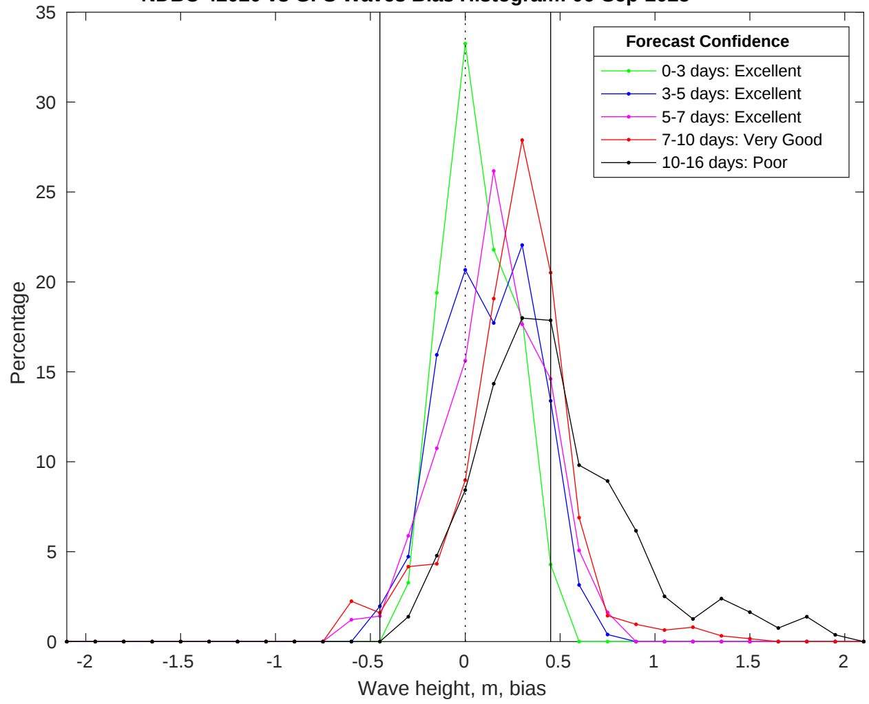
NDBC 42020 vs GFS Waves Bias Histogram: 06-Sep-2025
