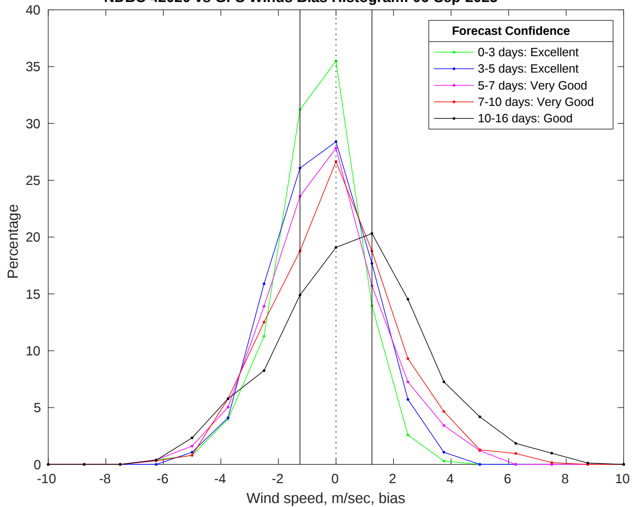
NDBC 42020 vs GFS Winds Bias Histogram: 06-Sep-2025
