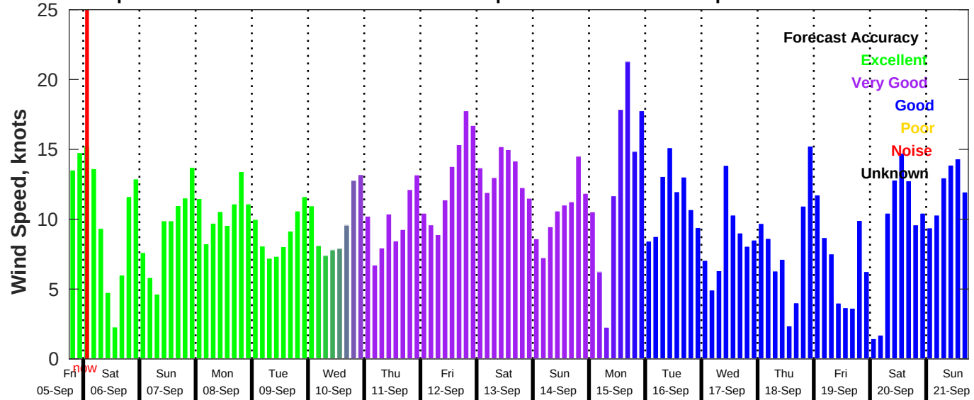
GFS Wind Speed Forecast for NDBC 42020 from 05-Sep-2025 18:00:00 to 21-Sep-2025 18:00:00
