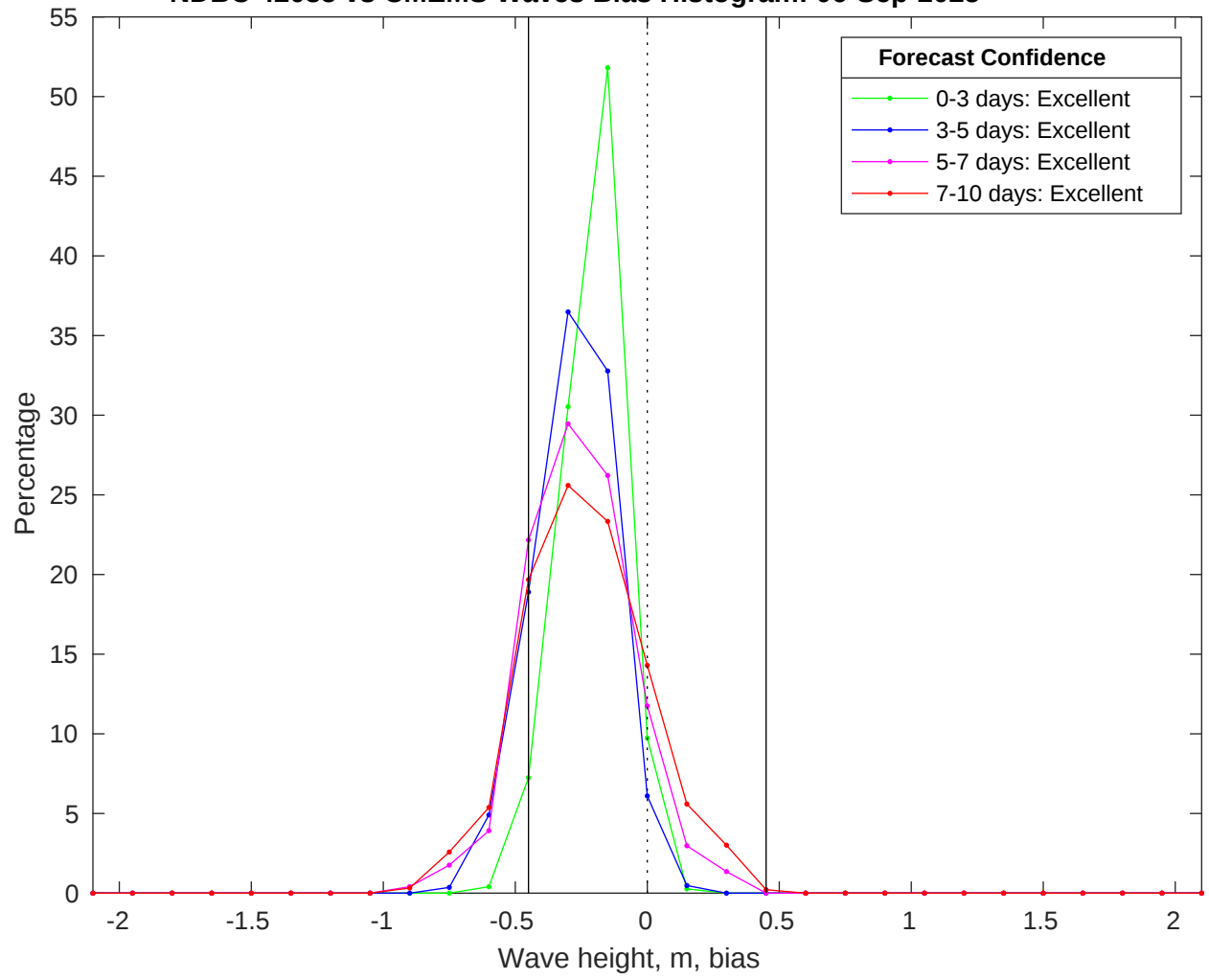
NDBC 42035 vs CMEMS Waves Bias Histogram: 06-Sep-2025
