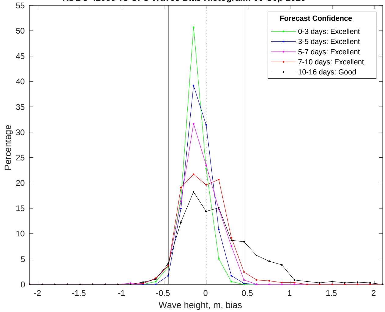
NDBC 42035 vs GFS Waves Bias Histogram: 06-Sep-2025
