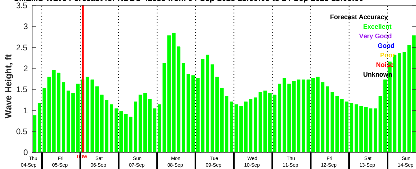
CMEMS Wave Forecast for NDBC 42035 from 04-Sep-2025 18:00:00 to 14-Sep-2025 18:00:00
