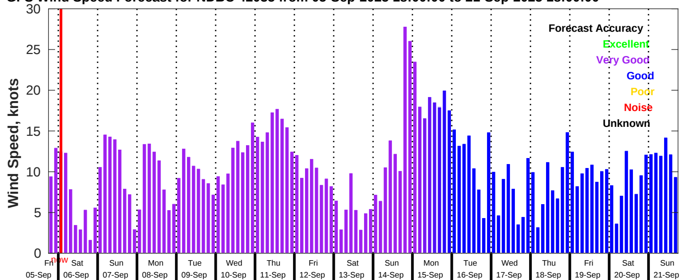
GFS Wind Speed Forecast for NDBC 42035 from 05-Sep-2025 18:00:00 to 21-Sep-2025 18:00:00
