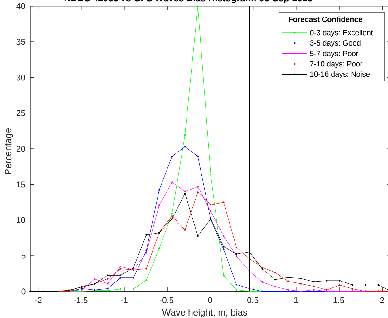
NDBC 42036 vs GFS Waves Bias Histogram: 06-Sep-2025
