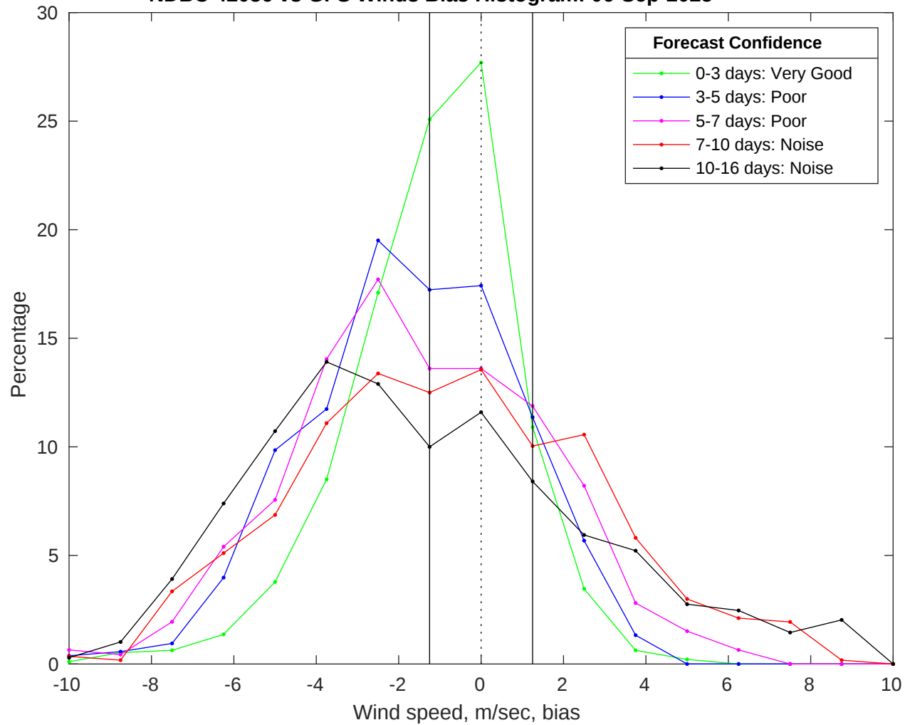
NDBC 42036 vs GFS Winds Bias Histogram: 06-Sep-2025
