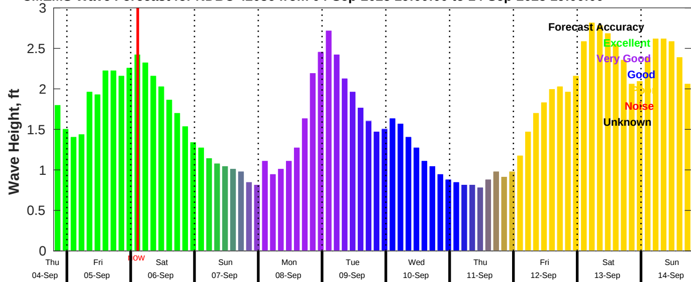
CMEMS Wave Forecast for NDBC 42036 from 04-Sep-2025 19:00:00 to 14-Sep-2025 19:00:00
