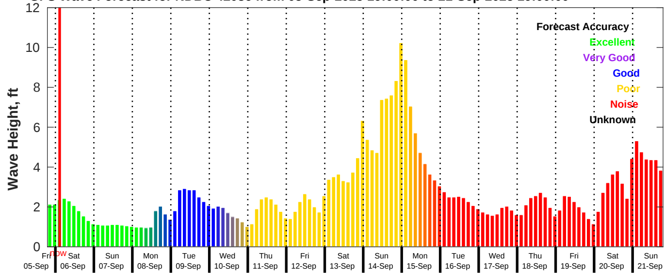
GFS Wave Forecast for NDBC 42036 from 05-Sep-2025 19:00:00 to 21-Sep-2025 19:00:00
