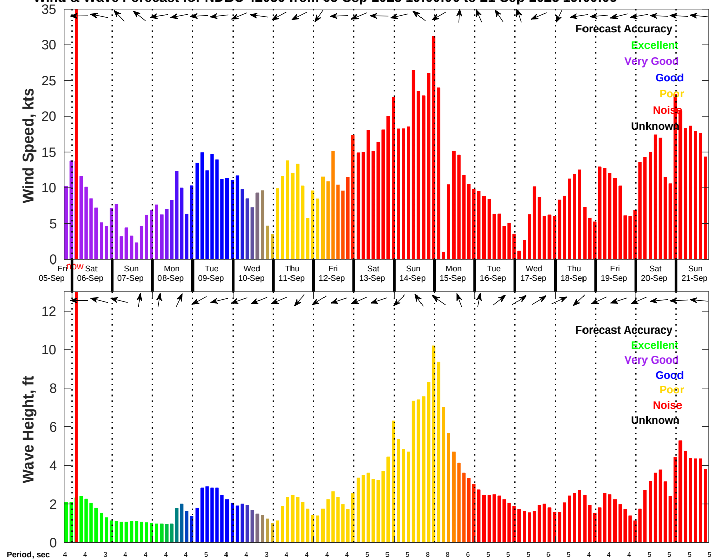
Wind & Wave Forecast for NDBC 42036 from 05-Sep-2025 19:00:00 to 21-Sep-2025 19:00:00
