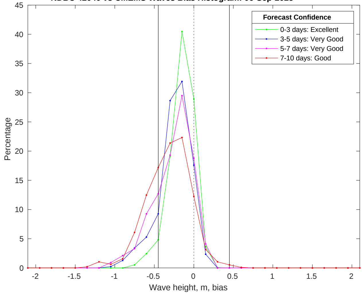
NDBC 42040 vs CMEMS Waves Bias Histogram: 06-Sep-2025
