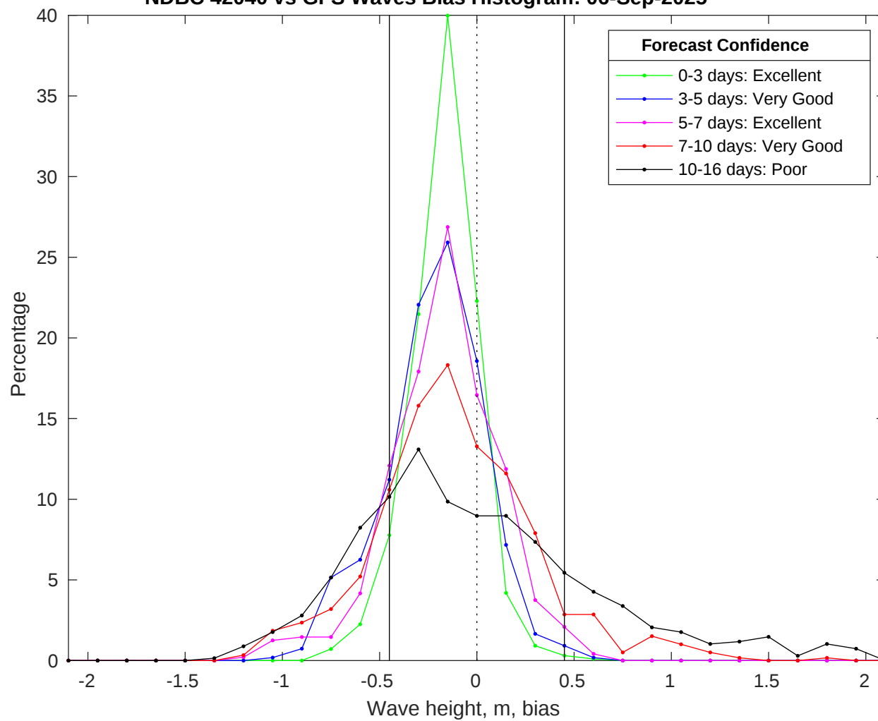
NDBC 42040 vs GFS Waves Bias Histogram: 06-Sep-2025
