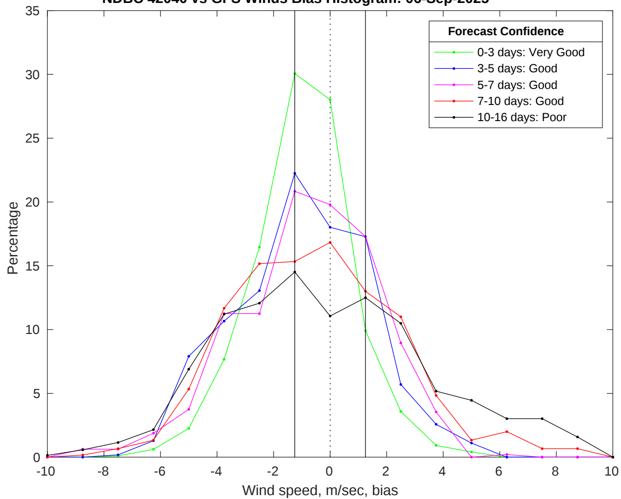
NDBC 42040 vs GFS Winds Bias Histogram: 06-Sep-2025
