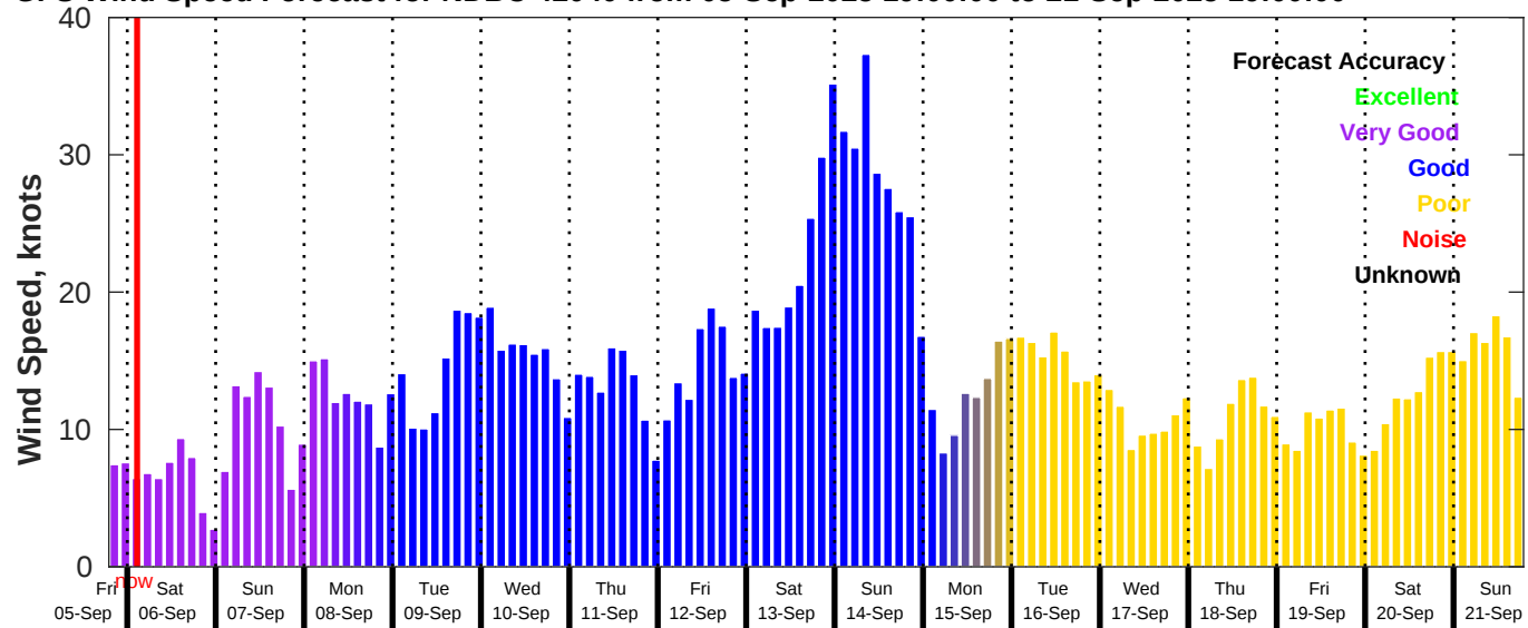
GFS Wind Speed Forecast for NDBC 42040 from 05-Sep-2025 19:00:00 to 21-Sep-2025 19:00:00
