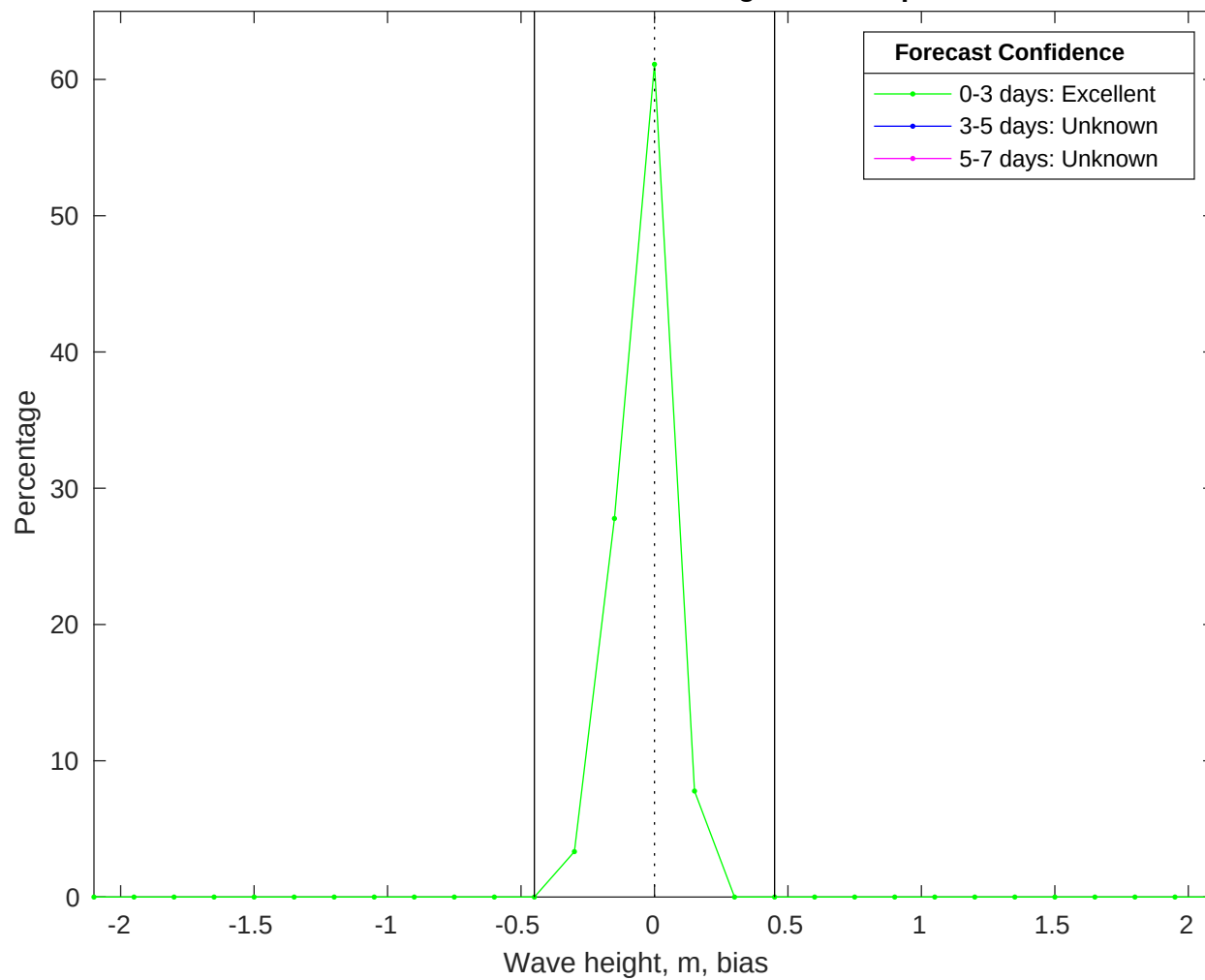
NDBC 44008 vs CMEMS Waves Bias Histogram: 06-Sep-2025
