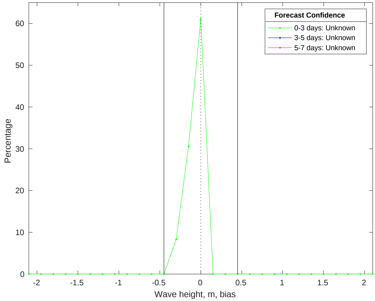
NDBC 44008 vs GFS Waves Bias Histogram: 06-Sep-2025
