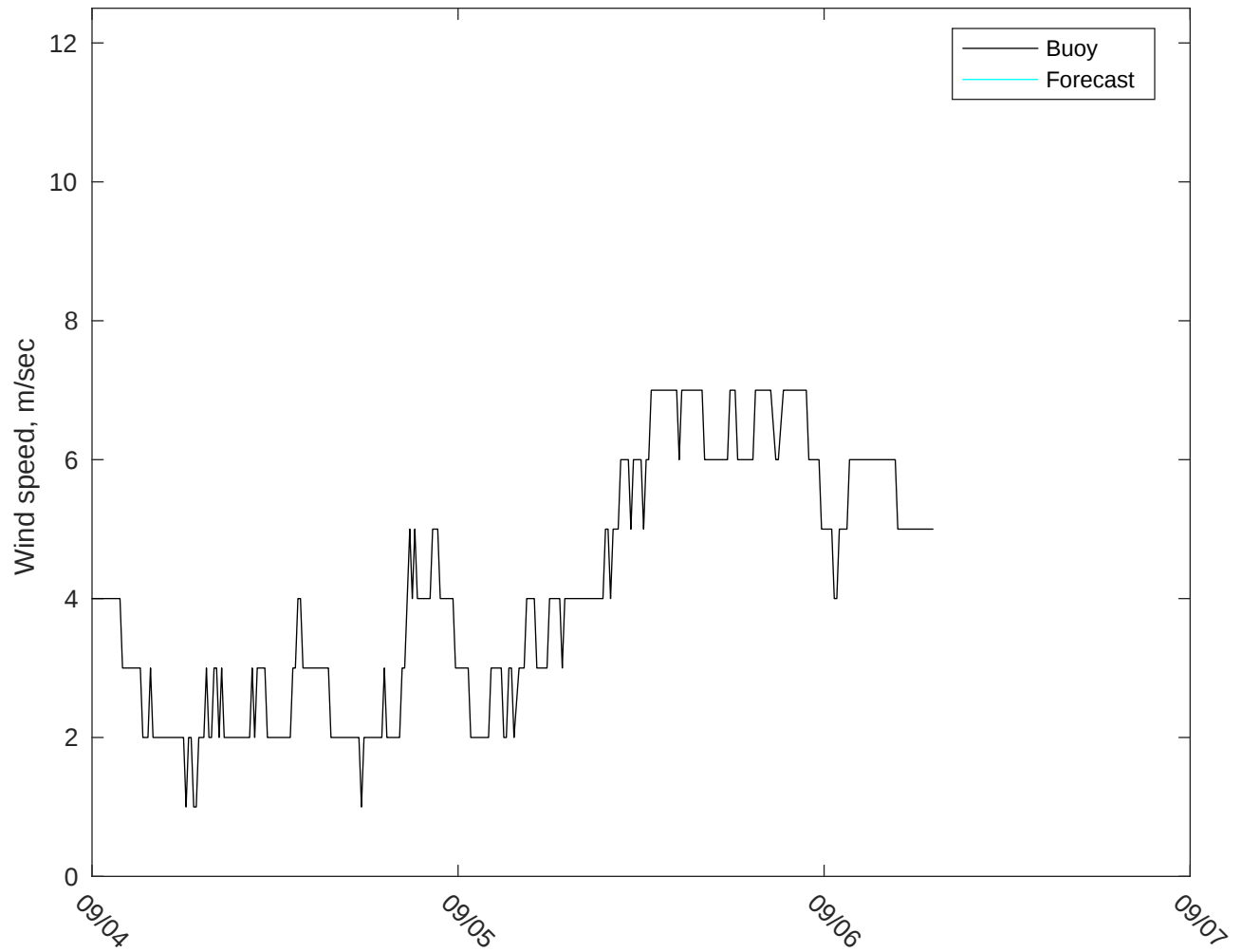
NDBC 44008 vs GFS Winds: 5 to 7 day forecast
